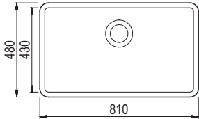
Nova Single bowl Ref. NOV N780 £452 Overall size: 810/480 mm Bowl size: 760/430/230 mm Cutout size: Template Available Minimum cabinet size: 700 mm Standard waste kit included
