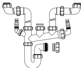
Space Saver Plumbing Kit for 1.5 and double bowl Ref. SSK2 £48
