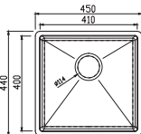
Jazz Single bowl Ref. JA012 £282 Overall size: 450/440 mm Bowl size: 410/400/190 mm Min cabinet size: 450 mm
