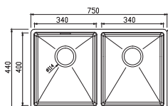
Jazz Double bowl Ref. JA024 £515 Overall size: 750/440 mm Bowl sizes: 340/400/190 mm Minimum cabinet size: 800 mm
