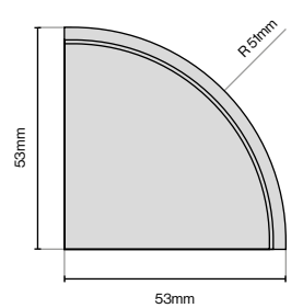
Under Cornice Quadrant (Smooth) 53mm (L) x 53mm (W) x 30mm (H)
