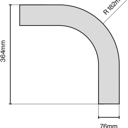
Curved Classic Cornice (Grained) 364mm (L) x 364mm (W) x 63mm (H)
