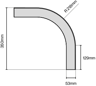
Curved Under Cornice (Smooth) 350mm (L) x 350mm (W) x 30mm (H)
