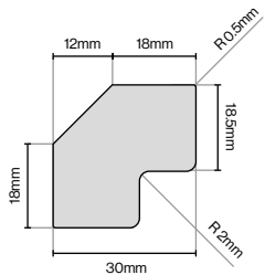
Corner Post 3050mm Lengths
