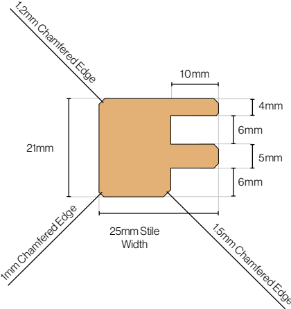
Brooklyn Oak Stile Cross Section
