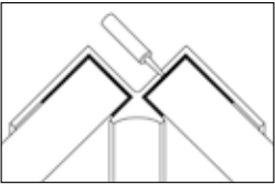
Internal corner Used on all internal 90° corners.
