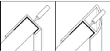
Finishing end trims and Quadrant trims Finishing end trims for panels.
