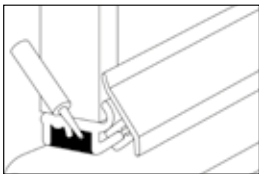
Seal one Sealant between seal & tray.
