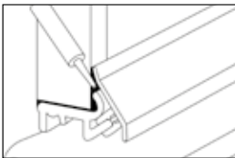
Seal two Panel encapsulated in sealant.
