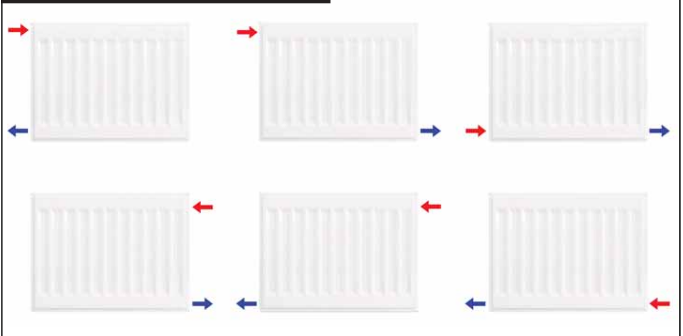
Connection Options for Compact Panel Radiators
